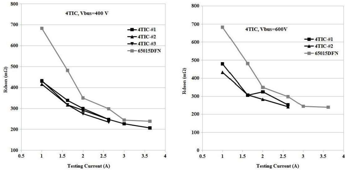
Dynamic Ron vs Testing Current @Vbus=400V, 600V
