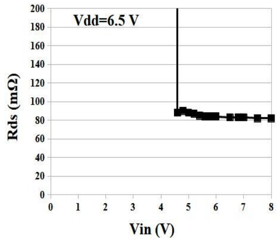
Static Rdson of 4TIC15DFV
