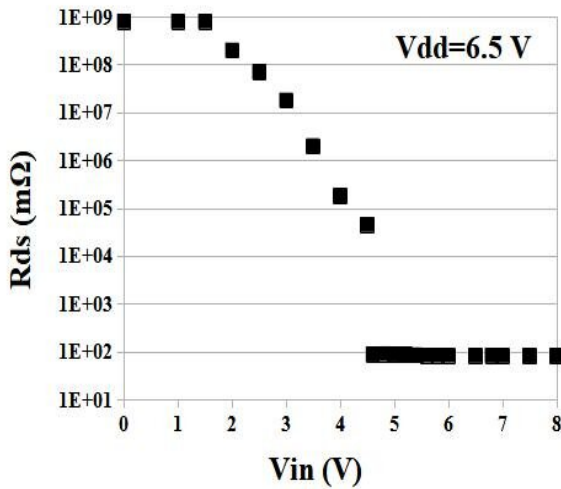
Static Rdson of 4TIC15DFV
